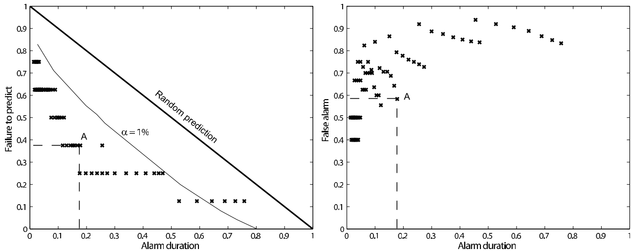
Figure 10. Error diagrams related to different combination of prediction parameters during the period May 23 to September 29, 2006. Parameters are varied as follows: 200 < C_{\Sigma} < 400 events per s days, 0.01 < \Delta < 1 day. s = 0.03 days. (left) Fraction of failure to predict ( f_p ) as function of alarm duration ( \tau ), black crosses; thin black line: 99% confidence level of the null hypothesis of random binomial predictions for the 24 large explosions in the considered period. The diagonal line corresponds to a random prediction. Deviations from this line depict the predictive power of the considered functional, i.e. the LP event rate. (right) Fraction of false alarms ( f_a ) as a function of alarm duration \tau , black crosses. Point A on the diagrams indicates a parameter combination allowing to predict 63% of Ubinas explosions with 17% of time covered by alarm and a 58% of issued alarms resulting false.
