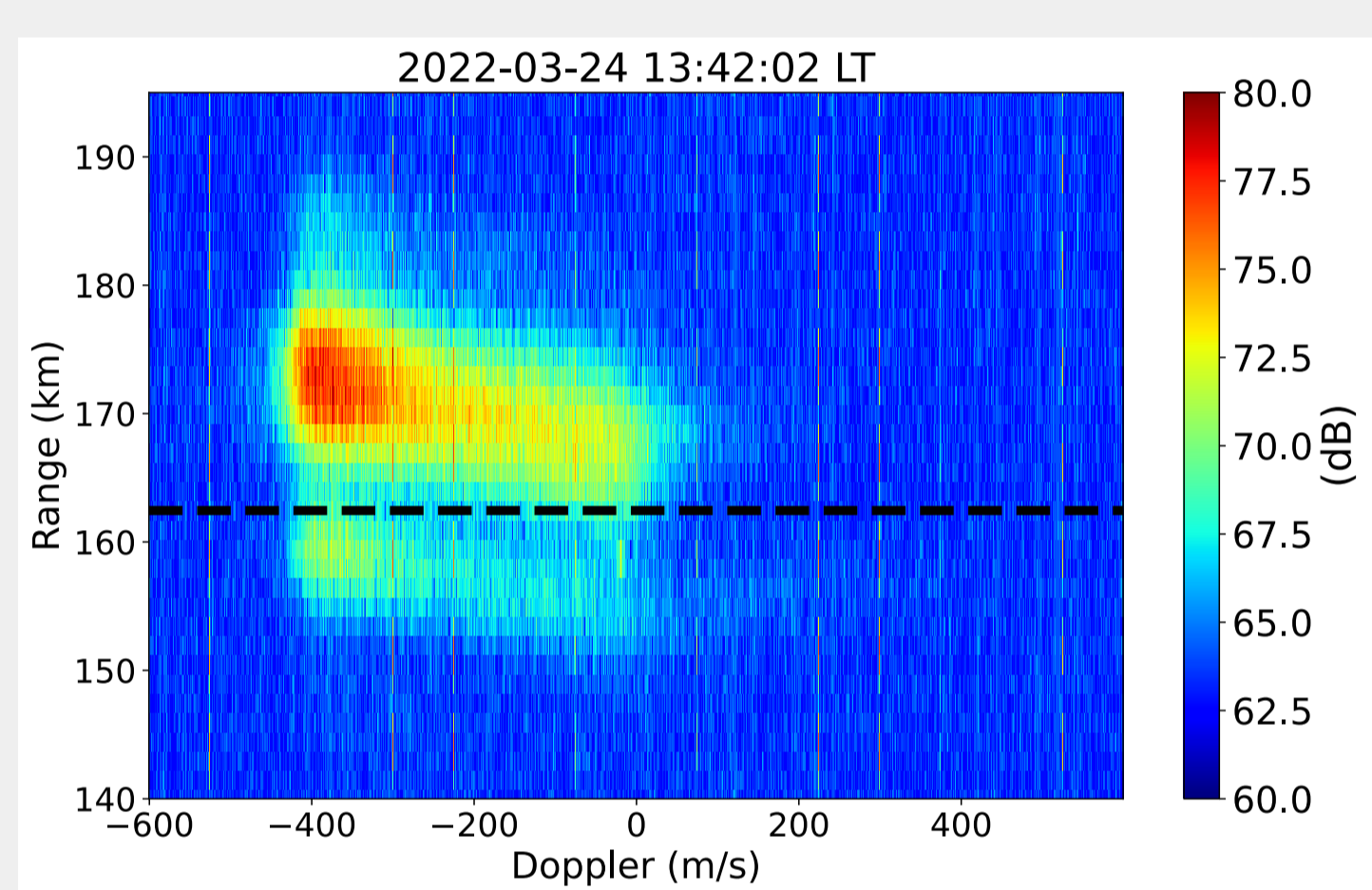
Figure 1. EEJ spectrum.
