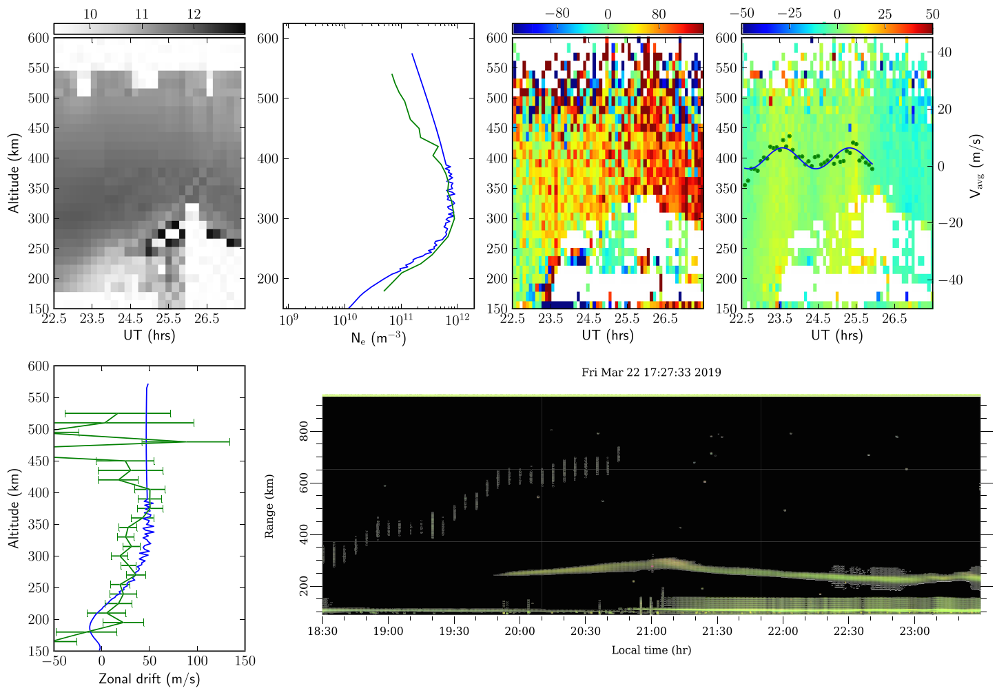
Figure 1. Incoherent scatter radar observations for 22 March 2019. (top row) Electron number density, electron density profile at 2300 UT (1800 LT), zonal plasma drifts, and vertical plasma drifts. (bottom row) Zonal plasma drift profile at 2300 UT (1800 LT), coherent scatter in range time Doppler intensity (RTDI) format. In this event, ESF plumes did not occur.
