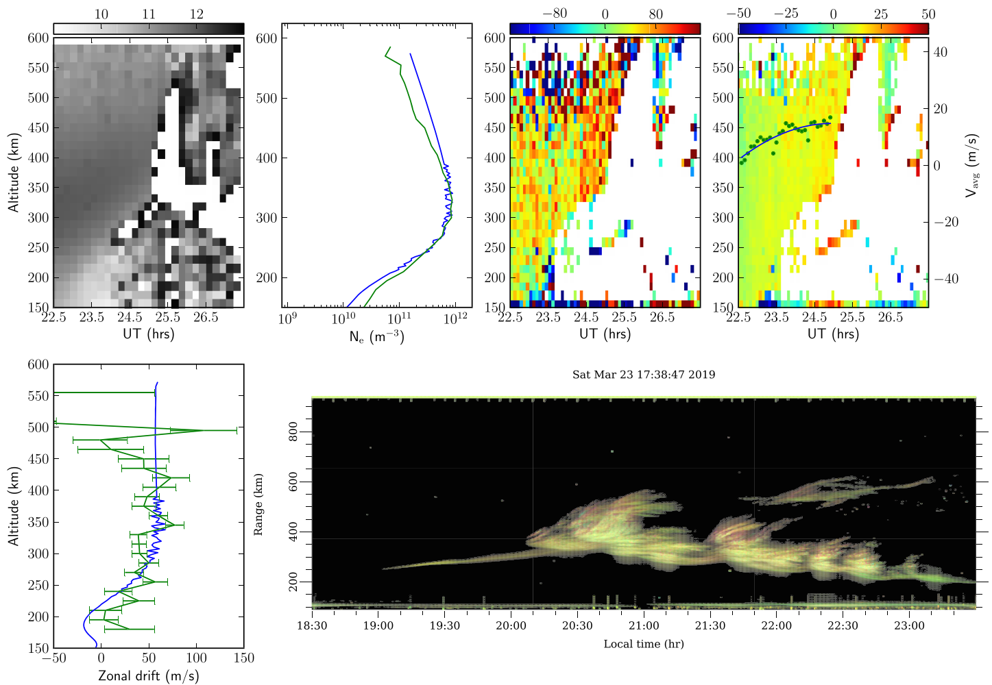
Figure 2. Same as Figure 1 except for 23 March 2019. ESF plumes were seen in this event.
