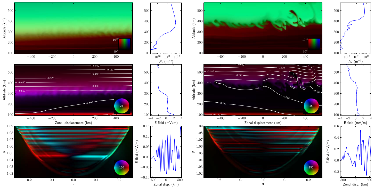
Figure 7. Same as Figure 6 except for 23 March 2019.
