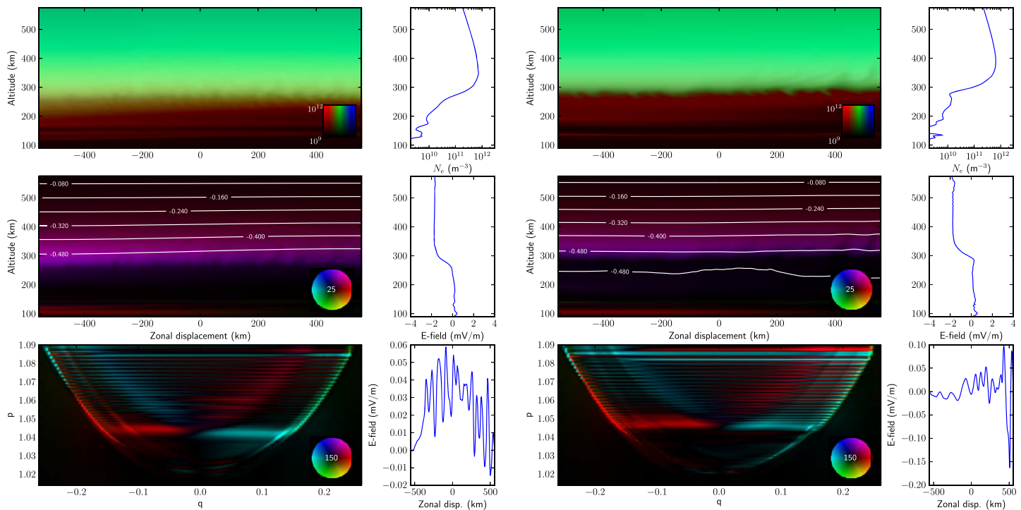
Figure 6. Numerical simulation of the 22 March 2019 ESF event. The simulation start time was 1800 LT (2300 UT). The left panel depicts conditions 60 min after the start or at 1900 LT (0000 UT), and the right panel 160 min after the start or at 2040 LT (0140 UT). The top panel in either case shows ion density, with red, green, and blue tones representing molecular ions, atomic ions, and hydrogen ions, respectively. A vertical cut of the electron density through the center of the simulation volume appears to the right. The middle panel shows equipotential lines superimposed on current density in the equatorial plane. The color wheel indicates the magnitude and direction of the current density, with full scale being 25 nA/m 2 . A vertical cut of the vertical electric field through the center of the simulation is shown to the right. The bottom panel shows current density in the meridional plane in magnetic coordinates ( p , q ). Full scale is 150 nA/m 2 . A horizontal cut of the zonal electric field through the center of the simulation is shown to the right.
