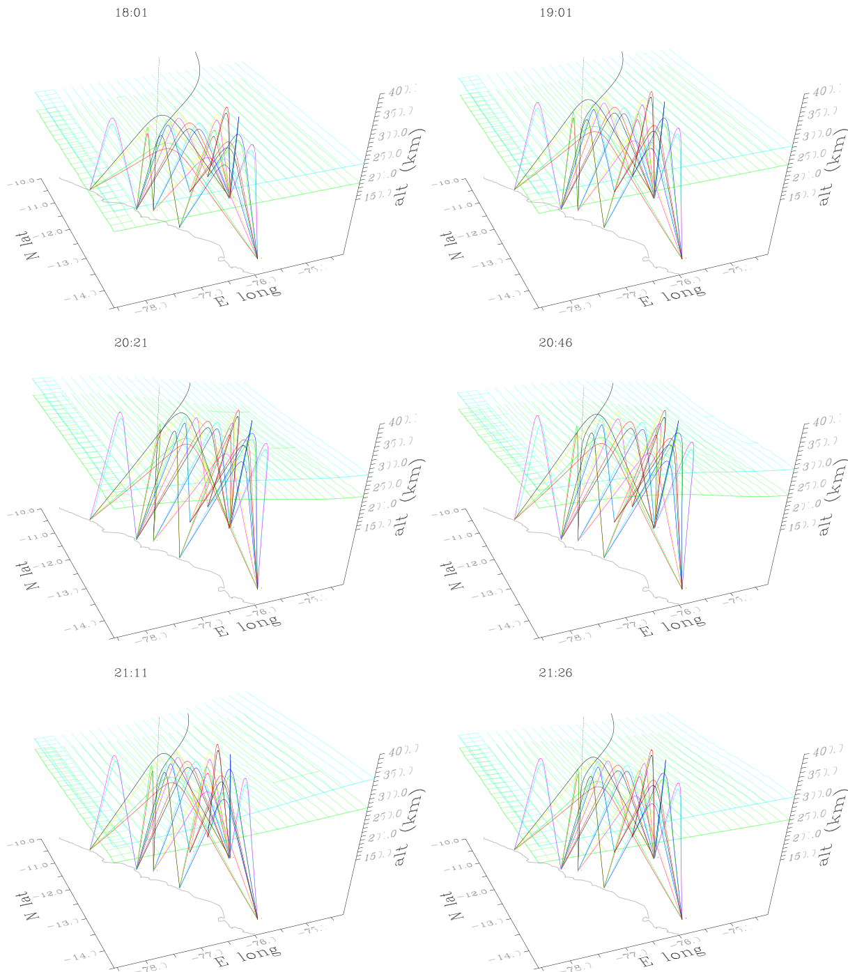
Figure 9. Same as Figure 8 except for 23 March 2019.
