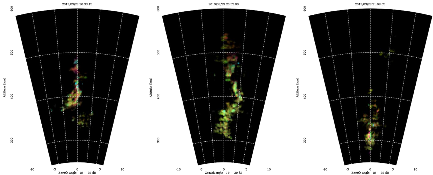
Figure 3. Aperture synthesis radar images of three closely spaced radar plumes that passed over the radar between 2030 and 2115 LT (0130–0215 UT).
