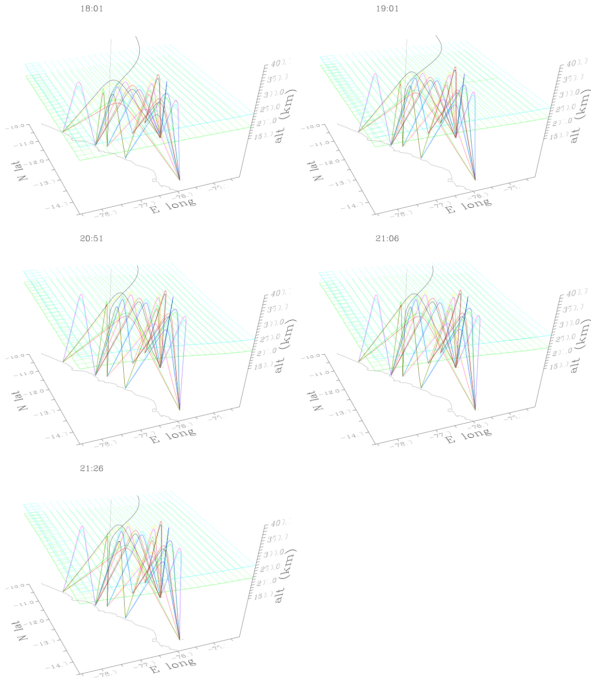
Figure 8. Ionospheric reconstructions deduced from HF beacon data for 22 March 2019. Each frame shows computed raypaths through a model ionosphere. The green and cyan meshes represent isodensity contours for N_e = 3E11 and 5E11 \text{ m}^{-3} , respectively. The black profile is an electron density profile at Jicamarca's location plotted on a linear scale.
