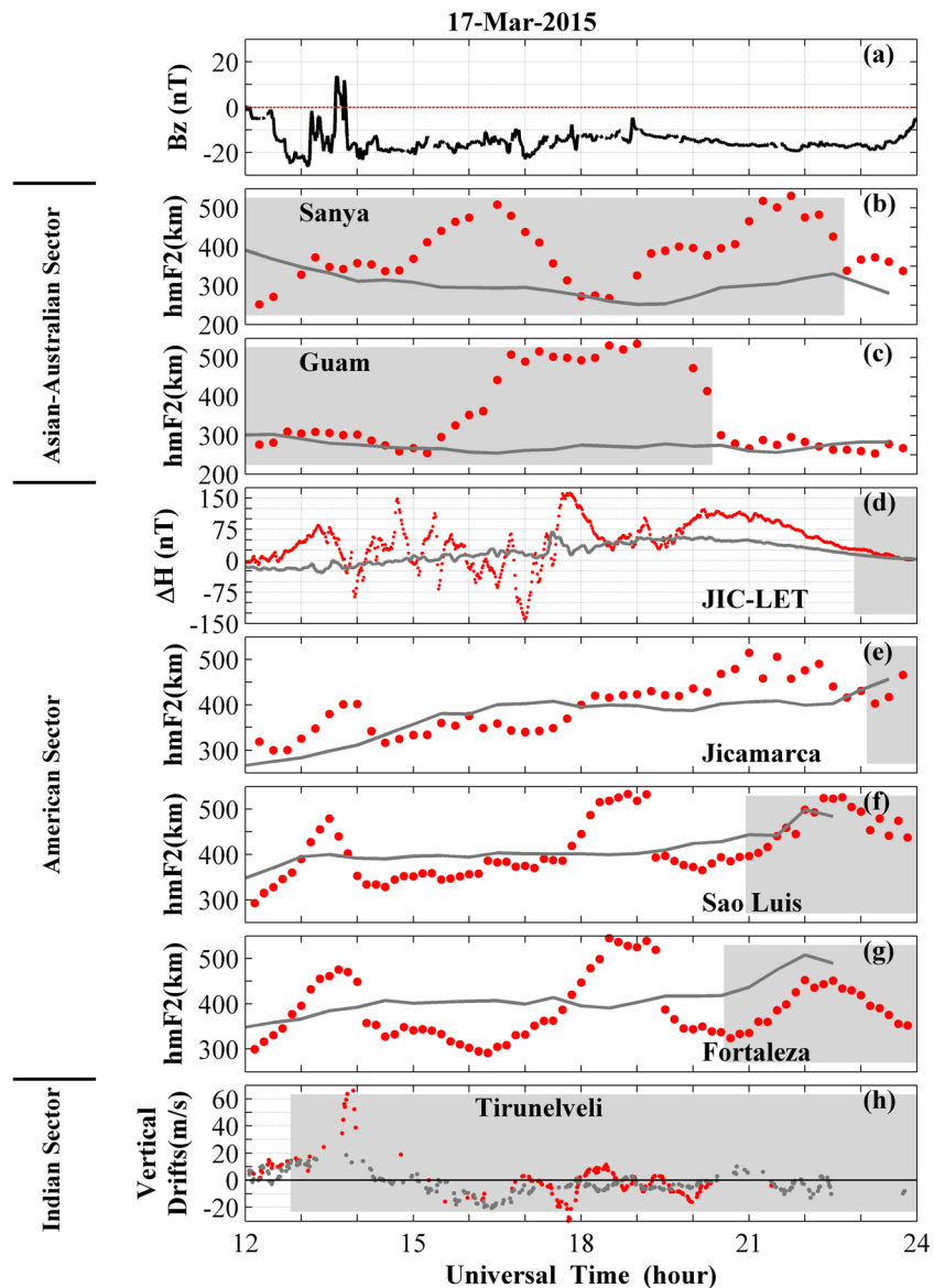
Figure 9. The variations of (a) IMF B_z ; (b and c) h_m F_2 at Sanya and Guam; (d) \Delta H_{jic-let} ; (e–g) h_m F_2 at Jicamarca, Sao Luis, and Fortaleza; and (h) the vertical Doppler drifts at Tirunelveli during 12:00–24:00 UT of 17 March. The gray curves of Figures 9b–9h denote the quiet time reference values of these parameters. The gray shaded areas indicate the period within 18:00–06:00 LT for each station.
