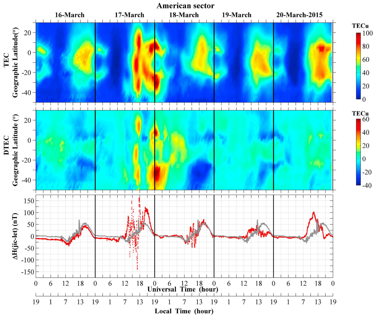
Figure 5. (top) The TEC and (middle) the deviations of TEC (DTEC) at longitude \sim 70^\circ\text{W} and (bottom) the variations of \Delta H_{\text{jic-let}} on 16–20 March 2015. The gray curve in Figure 5 (bottom) denotes the quiet time reference values derived from the \Delta H_{\text{jic-let}} on 16 March. The mean TEC data of five international quiet days of the month are used as the reference values to obtain the DTEC.
