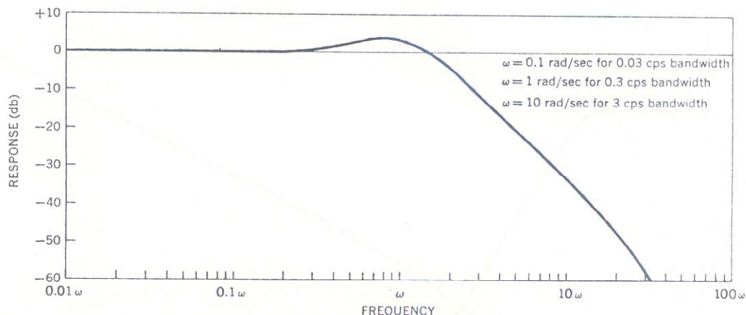
Figure 4—Normalized closed-loop frequency response
