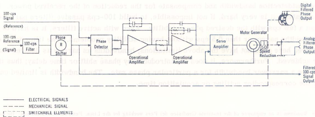
Figure 1—Phase-locked Phase Filter Block Diagram
