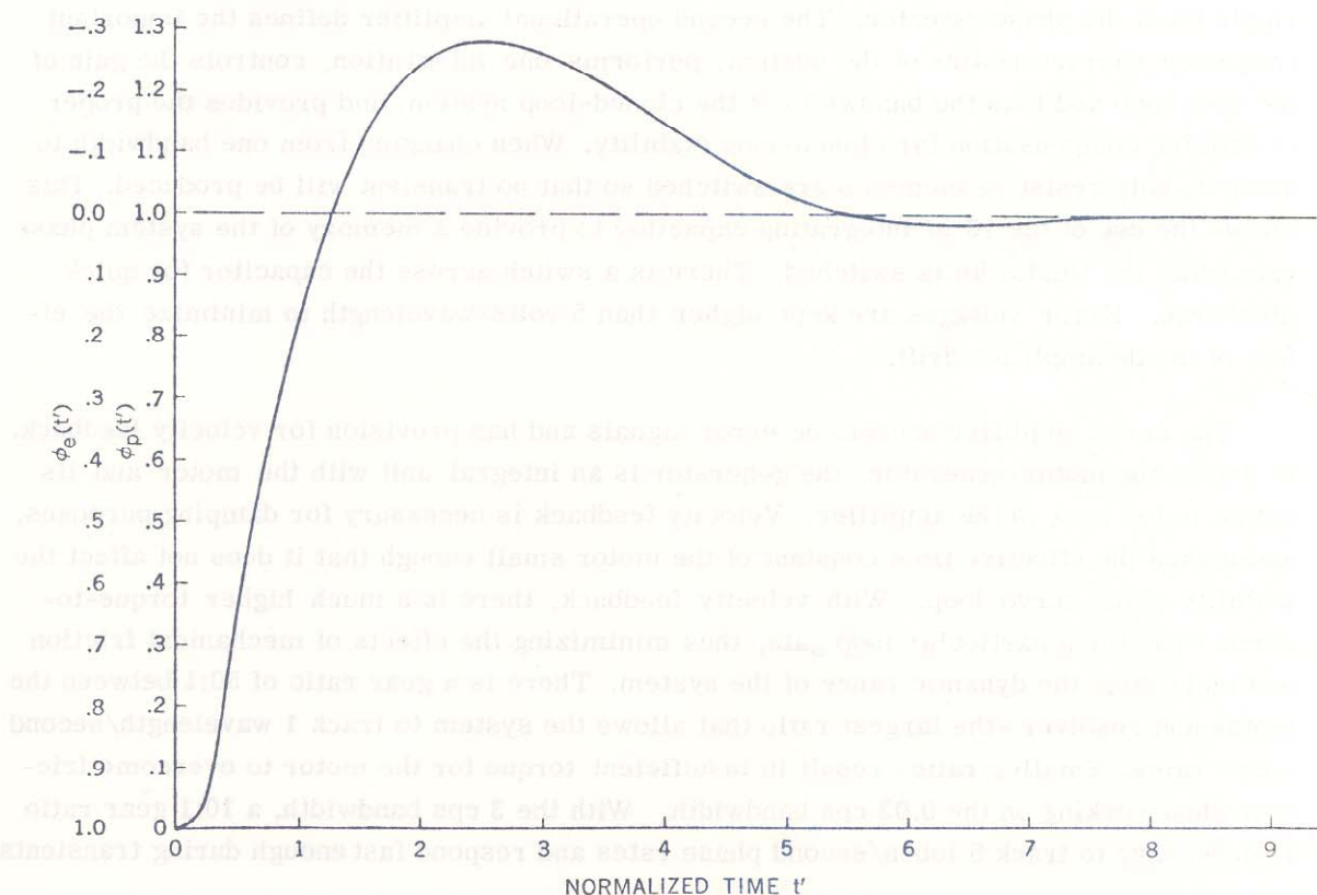
Figure 6—Step input response
