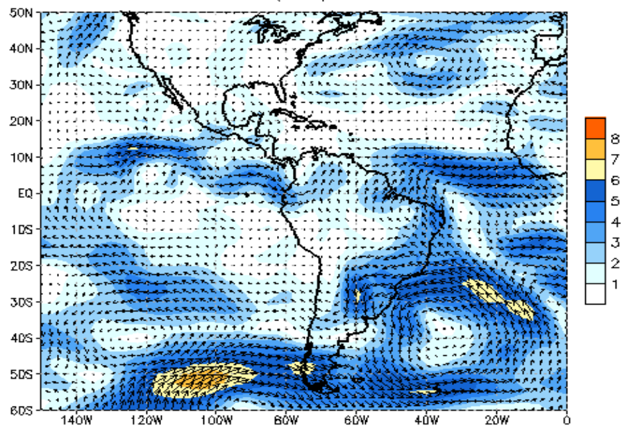
850 hPa Vector Wind Anomalies ( \text{ms}^{-1} ) 03 JUL 2017 – 01 AUG 2017
