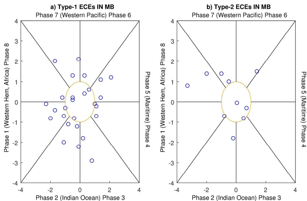
Figure 4. (RMM1, RMM2) phase space points for all Type-1 (a) and Type-2 (b) extreme cold episodes in the Mantaro basin. Eight defined regions of the phase space are labelled. ECEs in the Mantaro basin that are associated with a weak MJO are located inside the yellow circle. Analysis based on 1979-2010 period.
