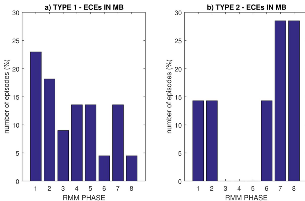
Figure 5. Histogram of the number of ECE's in the MB during each RMM Phase for (a) Type-1 ECE's and (b) Type-2 ECE's. Analysis based on Type-1 and -2 ECEs that occur during active MJO phases only (e.g., \sqrt{(2\text{RMM1})^2 + (2\text{RMM2})^2} \geq 1 ). Analysis based on 1979-2010 period.
