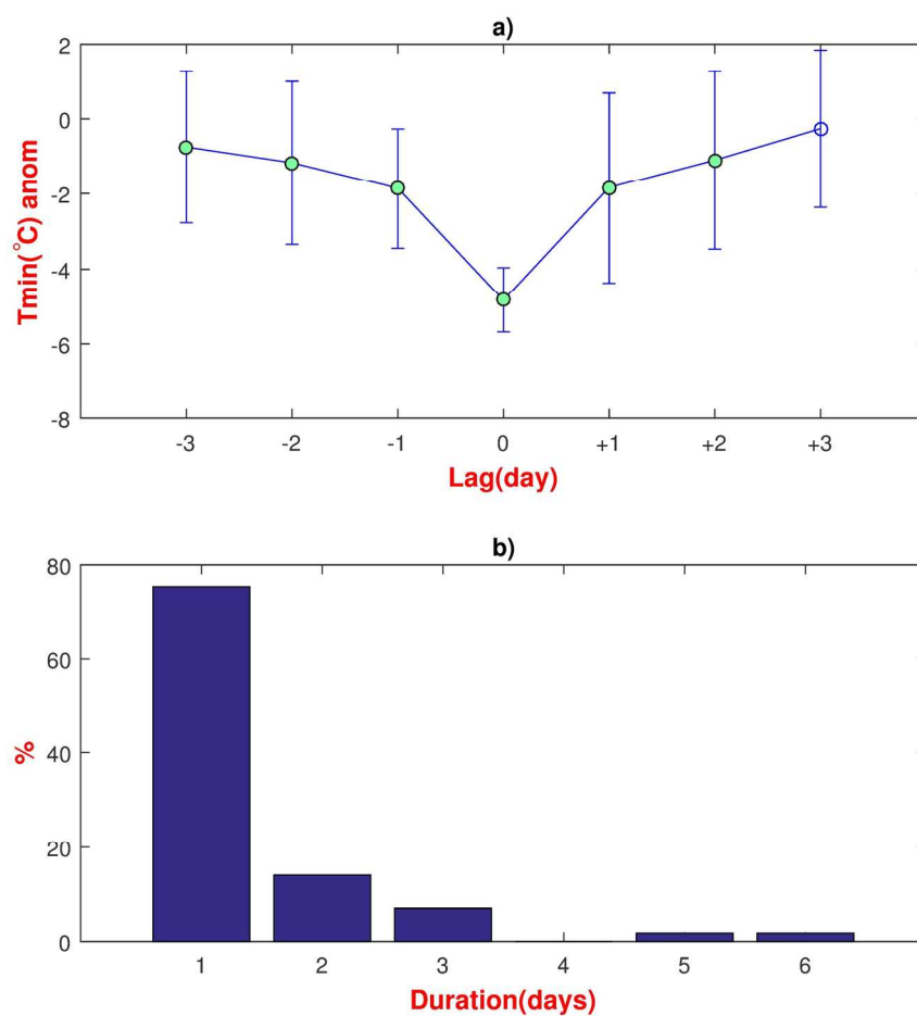
Figure 2. (a) Superposed epoch analysis applied to daily minimum temperature anomalies for extreme cold episodes in the central Peruvian Andes during austral summer (January-February-March). (b) Histogram of the duration of extreme cold episodes in the central Peruvian Andes during the austral summer. Green circles represent days where minimum temperature anomalies are statistically significantly different from zero at 95% confidence level based on Student's t-test. Data of minimum temperature of Huayao station was used in this study. Analysis based on the period 1979-2010.
