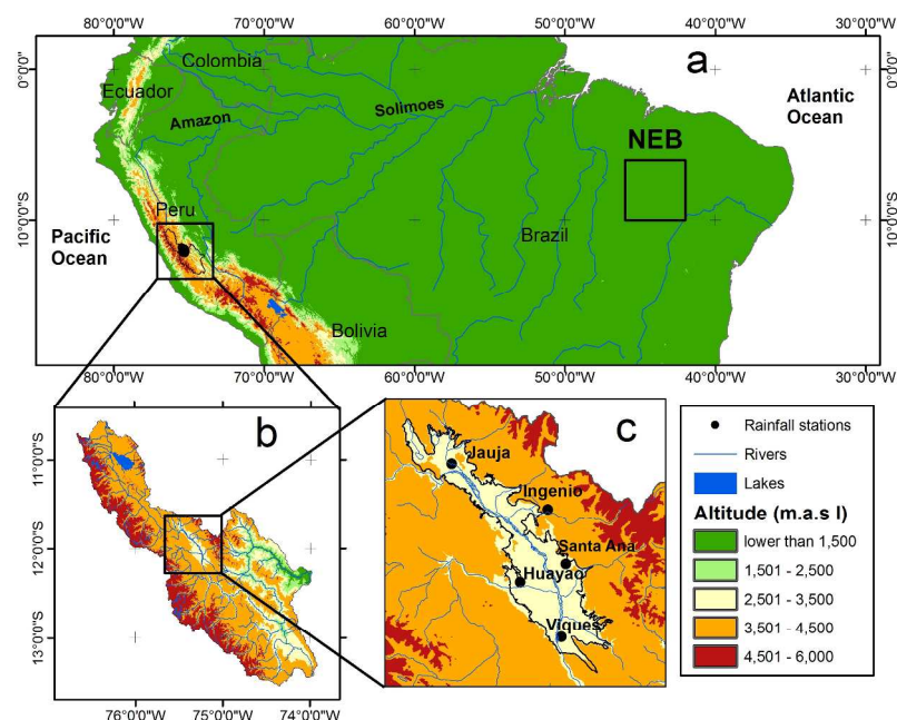
Figure 1. Location of Mantaro valley and all stations used in this study: a) South America, b) Mantaro basin, c) and Mantaro valley. The locations of all stations used in this study are represented by black circles. Black box represents the location of northeast Brazil.
