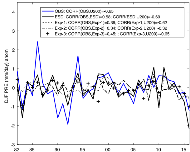
FIG. 11. Time series of the DJF precipitation anomaly index ( \text{mm day}^{-1} ; 1982–2016) for observations (blue line) and estimated by the ESD model (black solid line), Exp-1 (black dotted line), Exp-2 (black dash-dotted line), and Exp-3 (black plus sign). OBS represents the observed DJF precipitation anomaly index. U200 represents the observed DJF zonal wind anomaly index. The term CORR indicates Pearson correlation.
