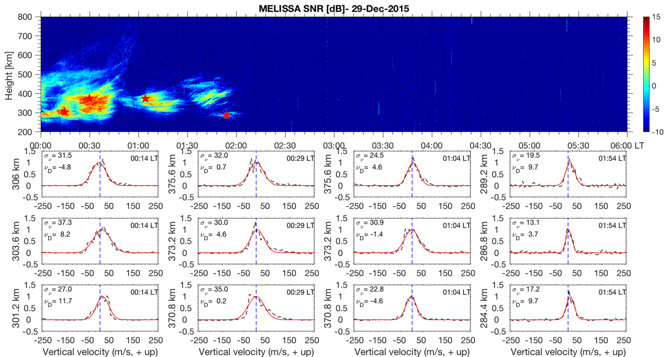
Figure 5. Same as Figure 4 but for 29 December 2015.
