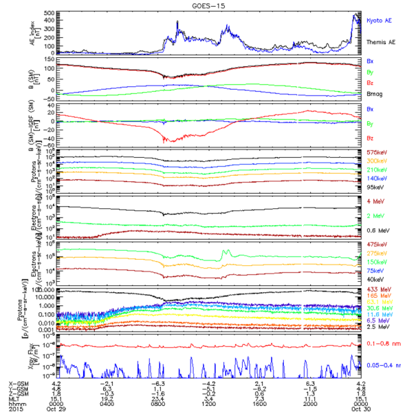
Figure 3. SEP event candidate to show isolated contribution on TEC measurements.
