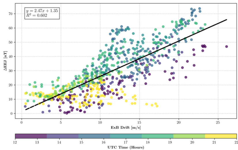
Figure 4. The linear correlation between the EEJ data and the E × B drift data was calculated on quiet days in order to evaluate the indirect estimation method.
