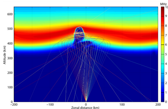
Figure 1. Radio wave dispersion associated with the Spread F phenomenon.
