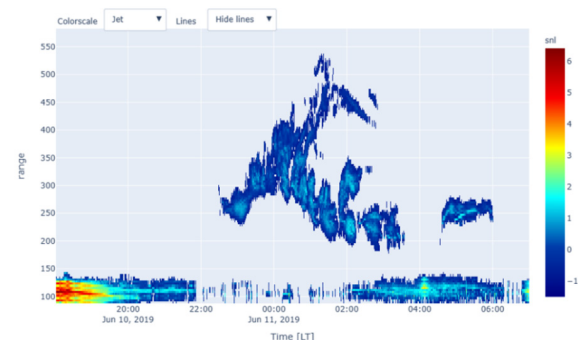
Figure 6. JULIA RTIs map.
