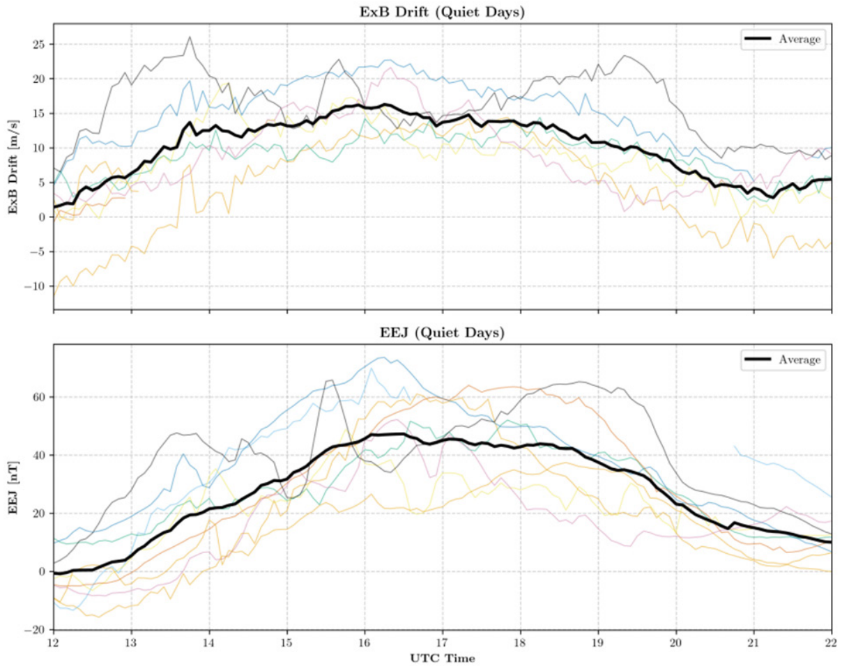
Figure 3. The E × B drift and the EEJ were calculated for a series of quiet days, and their average data (shown as the black line) was obtained.
