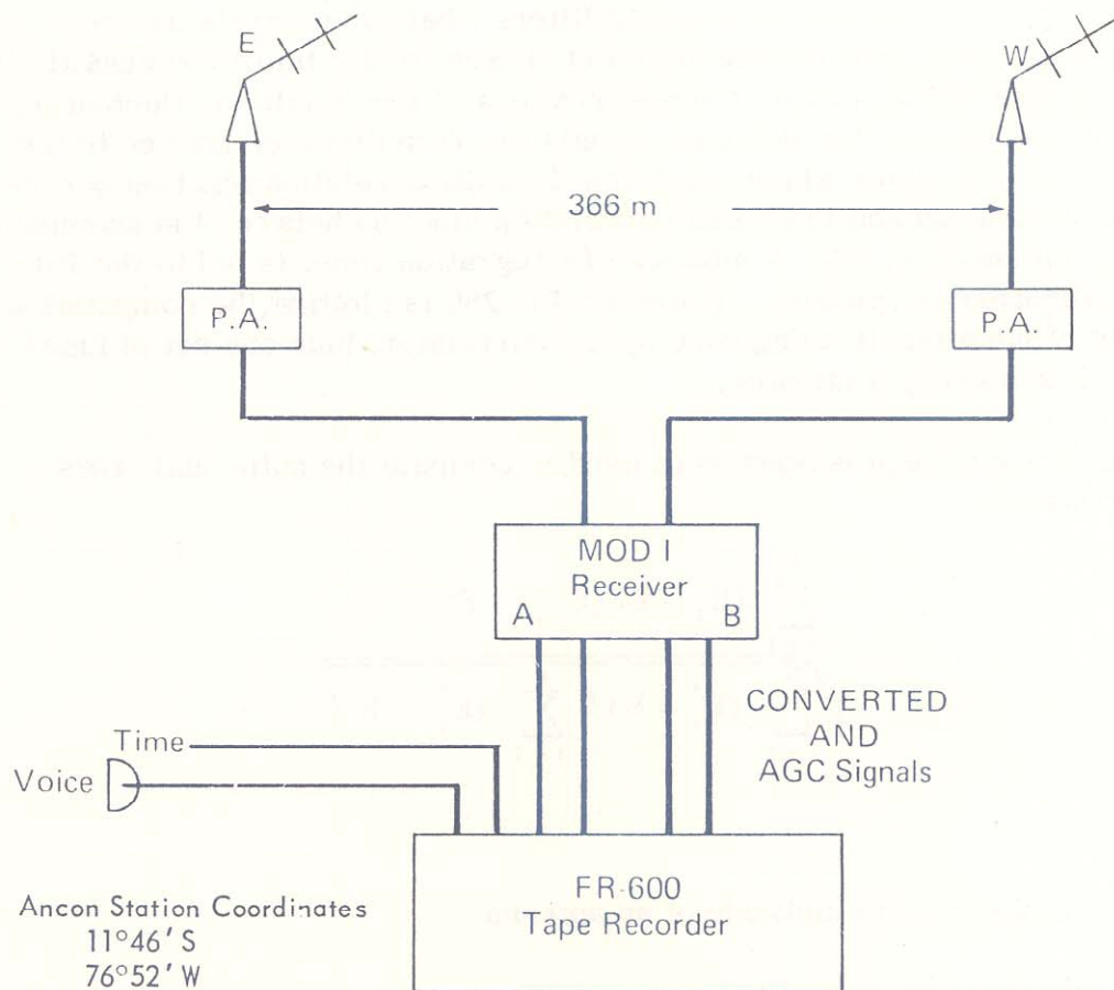
Figure 4. Block diagram of equipment used to gather scintillation data.
