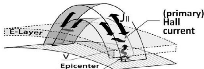
Fig. 11. Possible current closure through field-aligned current. The atmospheric motion ( V ) as the dynamo driver is assumed to be in the vertical direction for simplicity. The secondary Hall current is not depicted.
