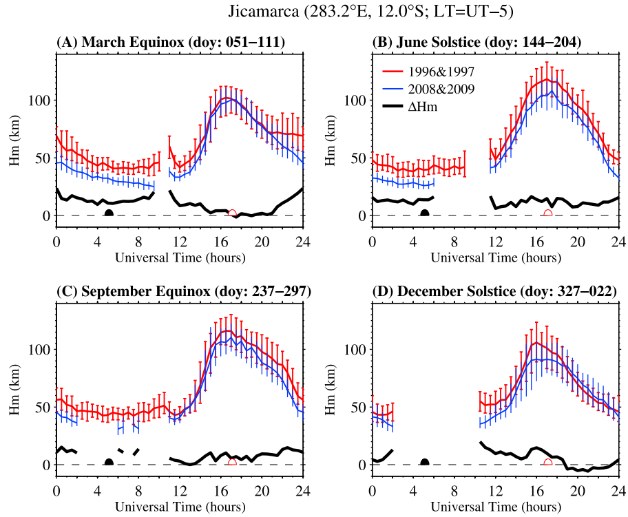
Figure 4. Universal time variation of H_m (F 2 layer Chapman scale height) over Jicamarca in four seasons for the last two solar minima. The red and blue lines indicate the seasonal median in 1996–1997 and in 2008–2009, respectively, and black lines show \Delta H_m , the differences of seasonal median H_m between 1996 and 1997 and 2008–2009. Bars show the upper and lower quartiles. The seasonal median and upper/lower quartiles are not calculated when the number of data is below 50 points (dotted line). The local midnight and noon at Jicamarca is also indicated by the solid and open semicircle, respectively.
