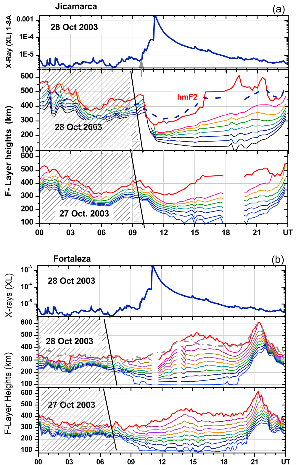
Figure 4. (a). The X-ray flux variations and the F layer heights at a number of sequential plasma frequencies, at 1 MHz interval, and the h_m F_2 , over Jicamarca on 28 October 2003, and on 27 October (a quiet day). (b). Similar plots for Fortaleza. The vertical slant line defining the end of the shaded region indicates the sunrise time as a function of height. The h_m F_2 on 27 October (dashed curve) is compared with that of 28 October in the middle plots for the respective stations. There is a data gap from 17:50 UT to 19:50 UT on 27 October at Jicamarca and at 1345 UT on 28 October over Fortaleza.
