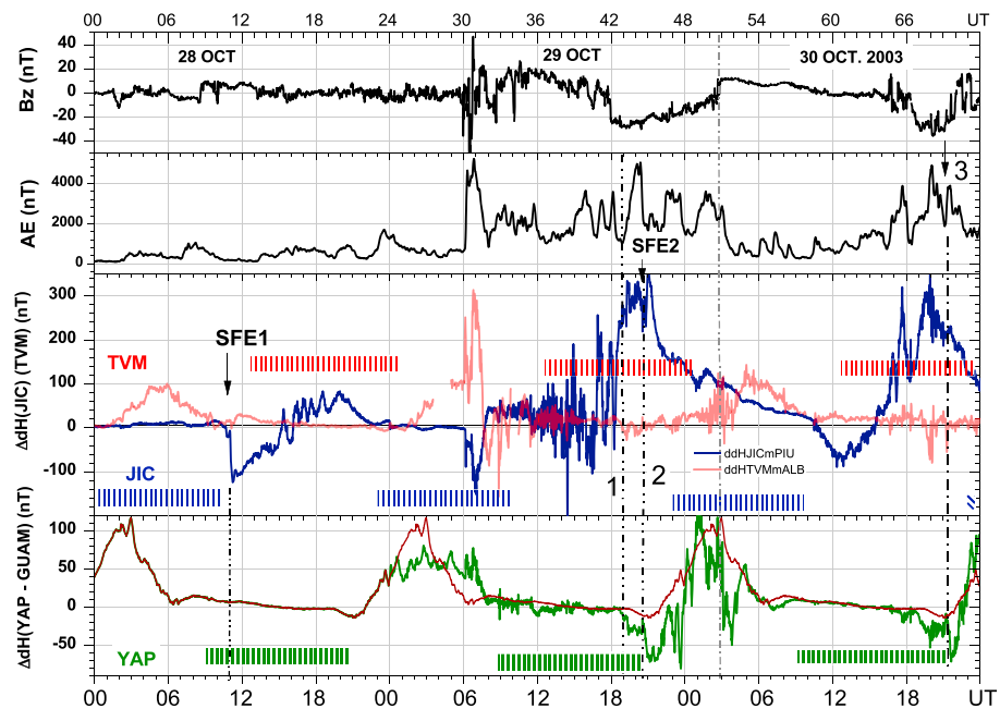
Figure 1. The variations in different parameters during 28 to 30 October 2003. (first panel) The interplanetary magnetic field component B_z and (second panel) the auroral activity index AE . (third and fourth panels) The magnetic field H -component variation over a dip equatorial station after subtracting the H variation over an off equatorial station (denoted as \Delta dH ), plotted for Jicamarca (navy blue), Trivandrum (red), and Yap (green). The responses to two solar flares are marked as SFE1 and SFE2, at 11 UT on 28 October and 2040 UT on 29 October, respectively. Night hours are indicated by vertical line straps (from the sunrise to sunset at 100 km) in the same color code as that of the data for the three stations. Please note that the UT and LT are related as LT = UT - 5 h for Jicamarca, LT = UT + 5:30 h for TVM, and LT = UT + 9:20 h for Yap.
