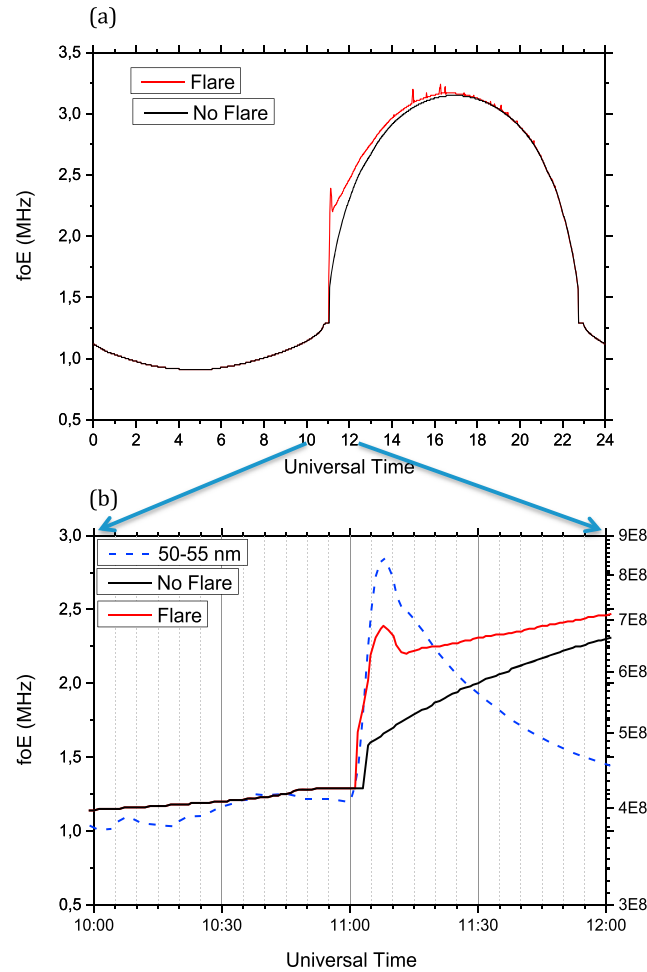
Figure 6. (a) SUPIM-INPE simulation of f_oE over Jicamarca on 28 October 2003. The red curve represents the f_oE variation when the ionizing radiation fluxes include those due to the X-class flare radiation, while the black curve represents the f_oE diurnal variation unaffected by the flare. The spiked peak in f_oE at 11 UT due to the flare may be noted. (b) An expanded time scale plot highlighting the f_oE increase due to the flare extra ionization. The flare emission variation in wavelength band 50–55 nm is also shown using rightside scale for which the axis values are photons \text{cm}^{-2} \text{s}^{-1} .
