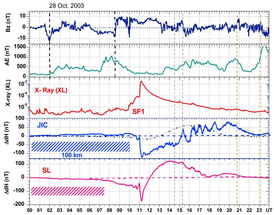
Figure 2. (first panel) The interplanetary magnetic field component B_z and (second panel) the auroral electrojet activity index AE variation on 28 October 2003. (third panel) The solar flare X-ray flux variation (in the 0.1–0.8 nm band) is shown. (fourth panel) The EEJ variation over Jicamarca represented by the parameter \Delta dH , which is the dH variation over Jicamarca (at the dip equator) from which the dH over the off-equatorial station, Piura, was subtracted. (fifth panel) The EEJ variation over the near dip equatorial station Sao Luis (SL), wherein Vassouras was used as the off-equatorial station. The slant line straps in blue and red for JIC and SL, respectively, indicate night hours ending at the E layer sunrise.
