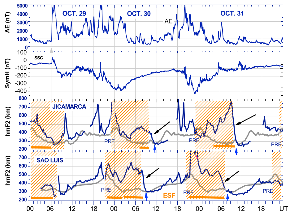
Figure 3. (first panel) Auroral activity (AE) index and (second panel) SYM-H (Dst) index variations during 29–31 October 2003. The F layer peak height ( h_mF_2 , blue curves) over (third panel) Jicamarca and (fourth panel) Sao Luis. The arrows point to the abrupt height decrease marking the DDEF polarity reversal to westward, consistently observed at both stations under the storm recovery phase on 30 and 31 October 2003. The grey curve represents the quiet time reference for h_mF_2 . The orange shaded intervals represent night hours, and the horizontal orange bars indicate the occurrence of spread F .
