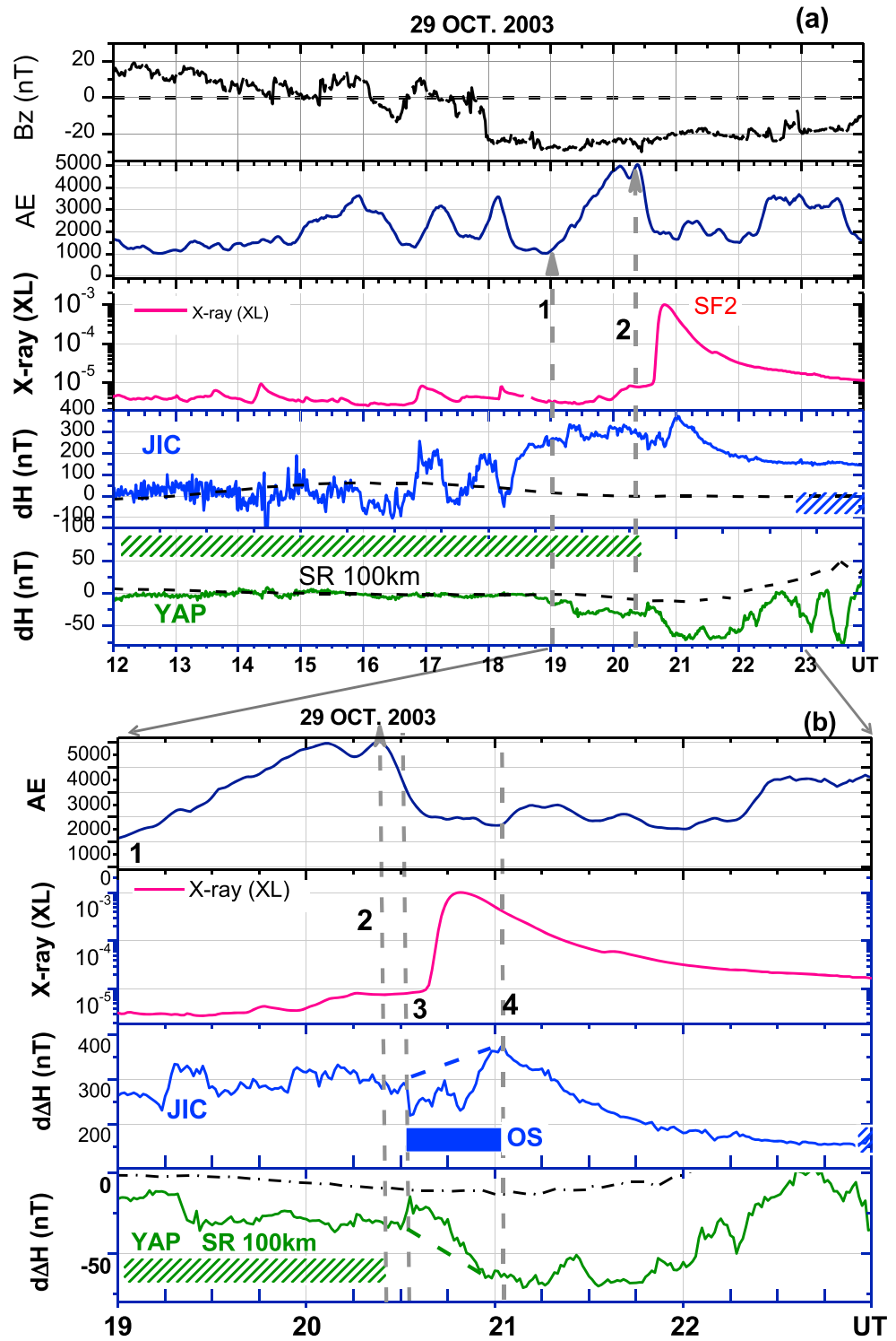
Figure 5. (a) The variation during 12–24 UT on 29 October 2003 of the B_z , AE index, X-ray intensity (0.1–0.8 nm band) (first to third panels) and \Delta dH over Jicamarca and Yap (fourth and fifth panels). (b) The same parameters as above plotted in a more expanded time scale during 19–23 UT. The dashed curves in bottom two panels in Figure 5a represent the quiet day curves for Jicamarca and Yap. The dash-dotted curve in the bottom panel of Figure 5b is the quiet day curve for Yap.
