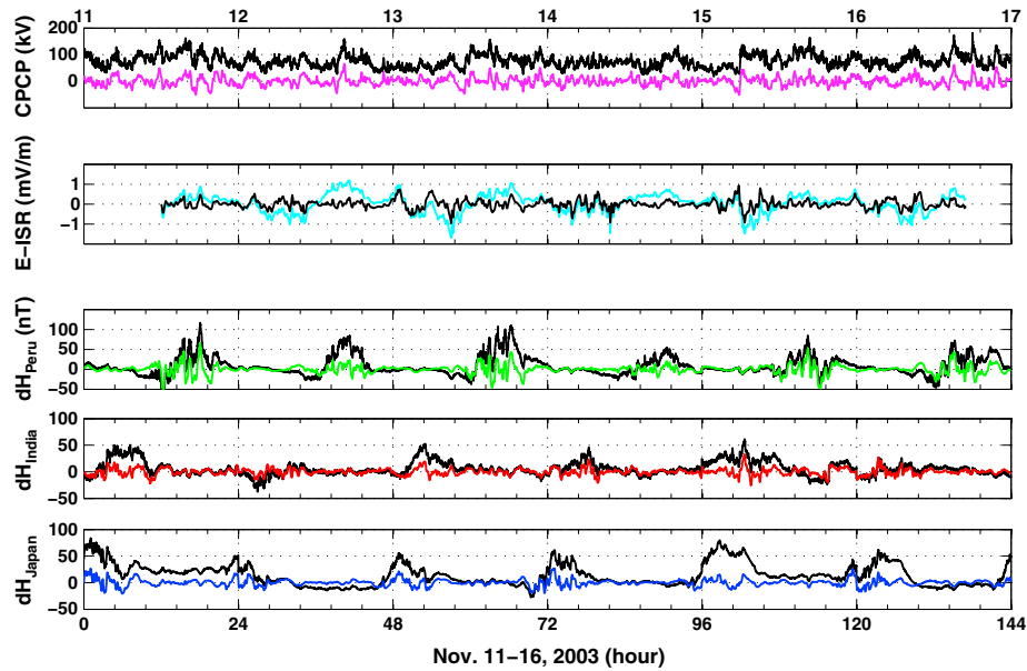
Figure 3. Original data and band-pass-filtered data during 11–16 November 2003. From top to bottom: CPCP derived by AMIE procedure, vertical drift measured by the JIC ISR (E-ISR), JIC-PIU \Delta H , TIR-ABG \Delta H , and YAP-BIK \Delta H . The original data are shown in black for CPCP and \Delta H values. For ISR vertical drift (second panel), the black color is used for filtered data. The color style for the filtered data applies to the other figures.
