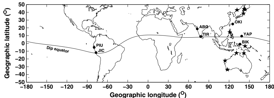
Figure 1. Locations of the geomagnetic stations listed in Table 1.
