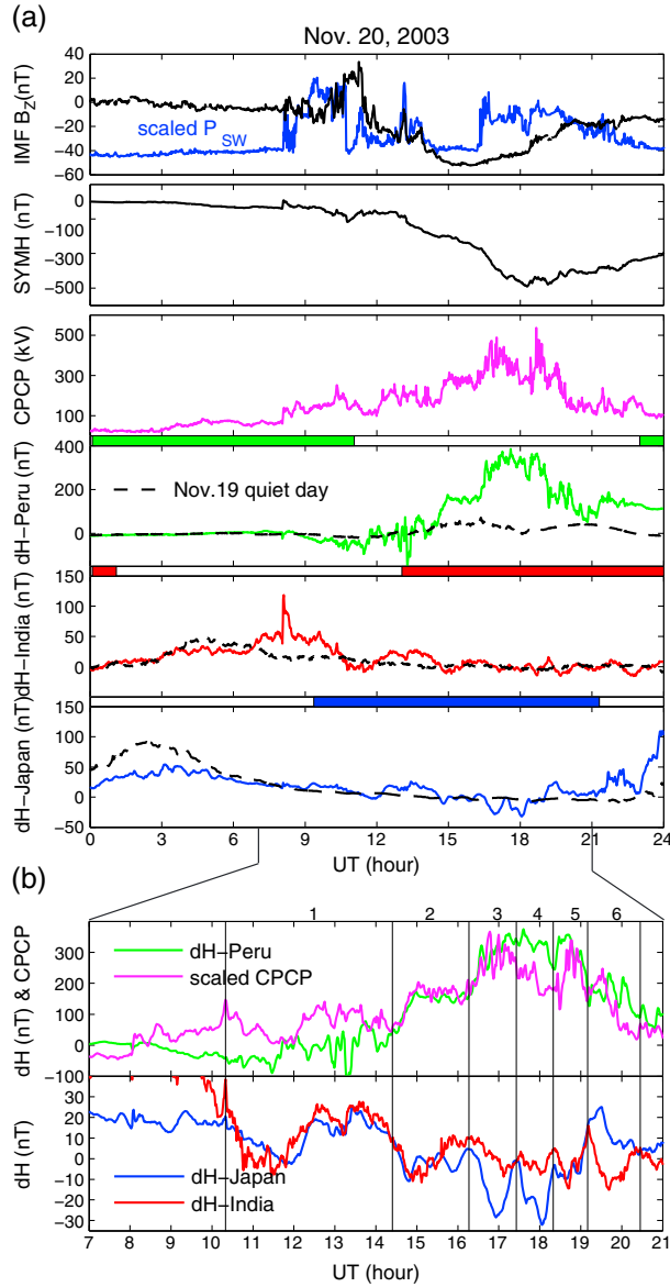
Figure 2. (a) In the first panel, the black line is IMF B_z and the blue line is the scaled solar wind dynamic pressure ( P_{sw} \times 3-50 nPa). The SYMH index is shown in the second panel and the CPCP calculated by AMIE procedure in the third panel. The \Delta H values inferred from the observations obtained using two geomagnetometers in Peru, India, and Japan are shown in the fourth, fifth, and sixth panels, respectively. The dashed line gives the quiet level measured on 19 November as a reference. The color/white bar illustrates the local nightside/dayside interval. (b) Comparisons of \Delta H in Peru and CPCP (first panel) as well as \Delta H values in Japan and India (second panel). The six intervals labeled by numbers are discussed in the text. The seven lines correspond to (from left) 1020, 1424, 1616, 1726, 1820, 1910, and 2027 UT.
