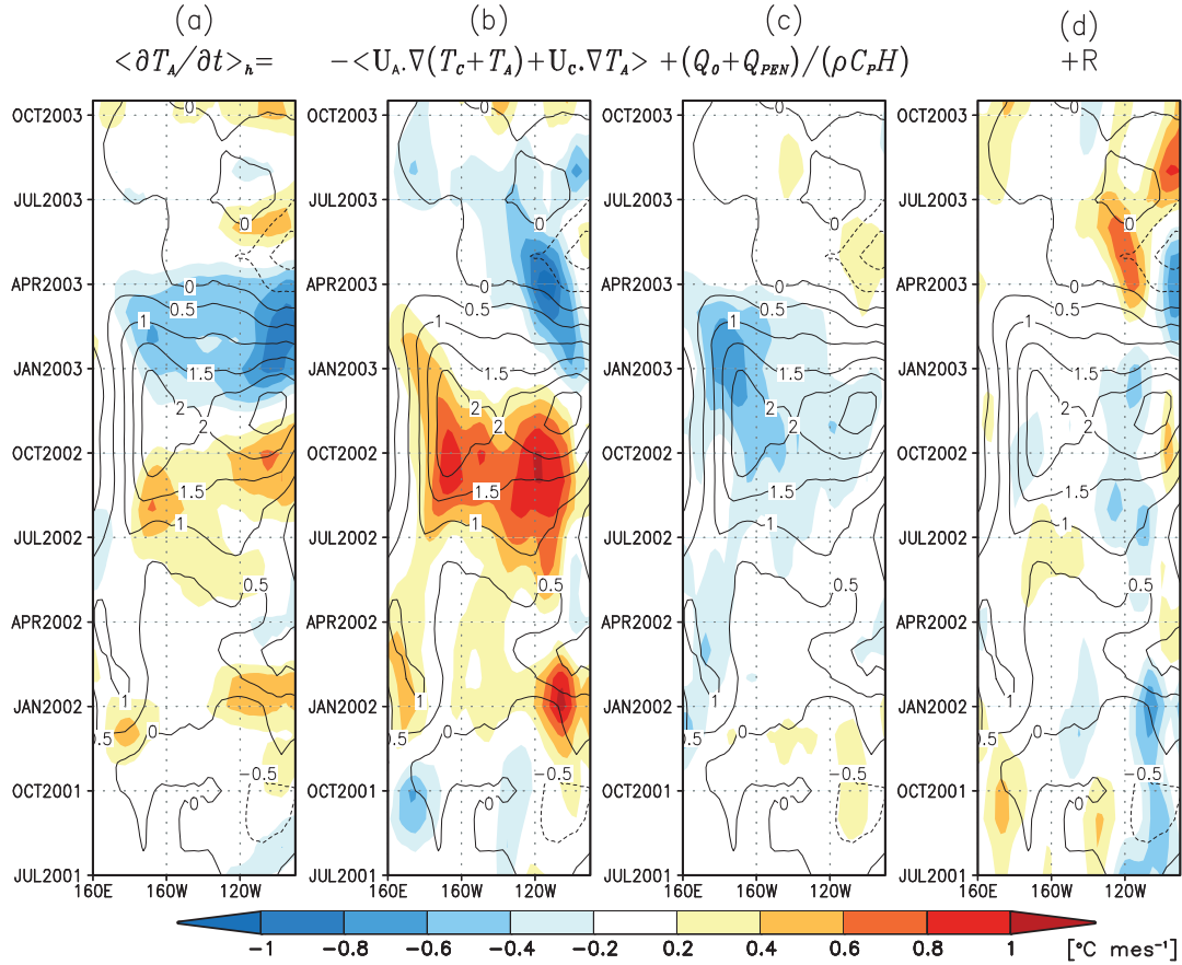
Figure 5. Evolution of the tendency terms (in colors) along the equator as defined in equation (1). (a) The rate of SST changes ( \langle \partial T_A / \partial t \rangle_h ). (b) The advection terms, which means the sum of the first three terms on the right-hand side of equation (1). (c) The surface fluxes [fourth term of equation (1)]. (d) The residual term ( R' ) that accounts for vertical mixing or entrainment. In each panel the SSTA is overlaid in black contours.
