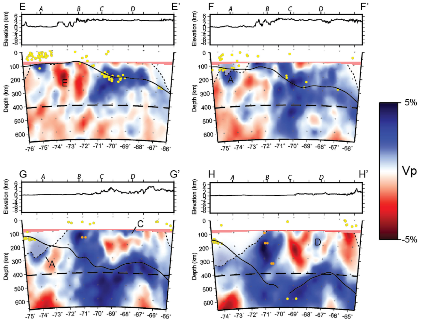
Figure 10. Trench parallel cross-sections through the V_p tomography model. Cross-section locations are as shown in Fig. 1. Dashed lines are the same as in Fig. 6. Intersection with trench perpendicular cross-sections indicated by italicized letters A, B, C and D. Yellow dots are earthquake locations from the EHB catalogue (Engdahl et al. 1998). Solid black line marks the top of the Nazca slab from the Slab1.0 model (Hayes et al. 2012). Orange dots mark reflection points from James & Snoke (1990). Labelled anomalies (A, C, D and E) are discussed in the text. Cross-sections through the V_s tomography model are shown in the Supporting Information Fig. S11.
