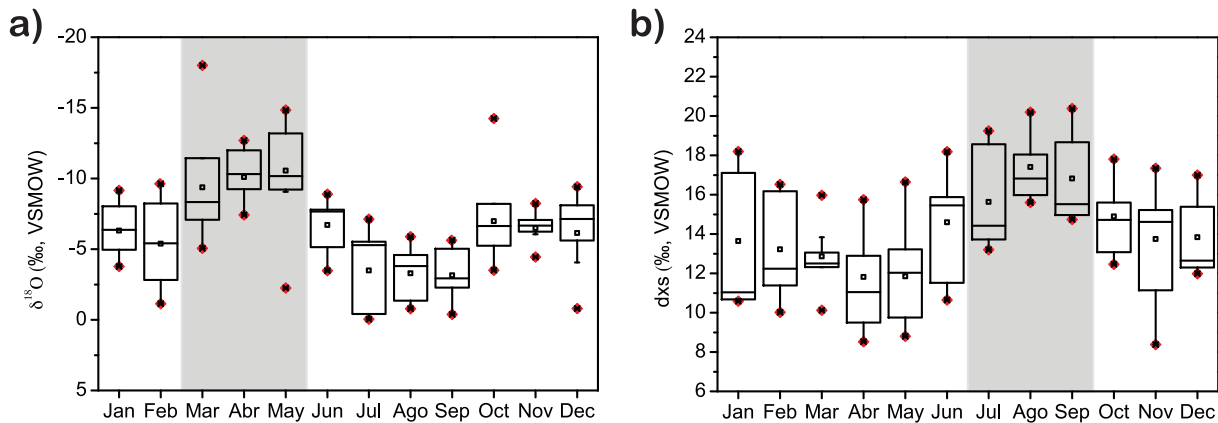
Figure 5. Boxplot of monthly (a) \delta^{18}\text{O} and (b) dxs of precipitation at the Palestina station based on biweekly sampling.
