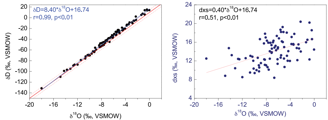
Figure 4. (a) \delta^{18}\text{O} and \delta\text{D} of precipitation at the Palestina station on a bi-weekly time step. The GMWL is represented by a solid red line and deviations of \pm 5\text{‰} are represented with dashed lines. (b) Correlation between of \delta^{18}\text{O} and \text{dxs} of precipitation at the Palestina station on a bi-weekly time step.
