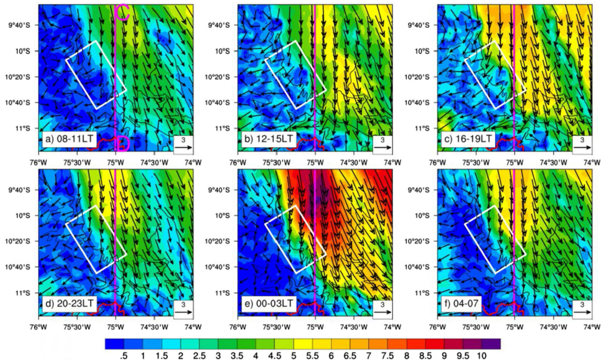
Figure 12. Vector field and magnitude of horizontal winds (m/s) at 730 hPa for the black box in figure 11. The white box represents the PEI hot-spot region (see figure 4f). Line C–D (magenta line) shows the variation in latitude set at 75°W longitude for figure 15.
