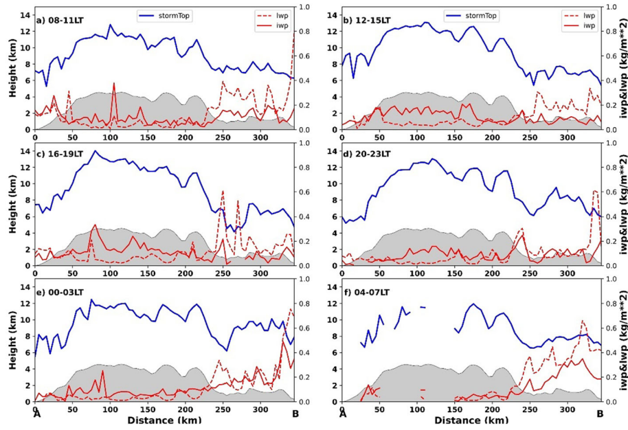
Figure 6. Similar to figure 5, but for total tropospheric hydrometeors (red dashed line is LWP, solid red line is IWP) and cloud top (blue line). (a) 08–11 LT, (b) 12–15 LT, (c) 16–19 LT, (d) 20–23 LT, (e) 00–03 LT, and (f) 04–07 LT.
