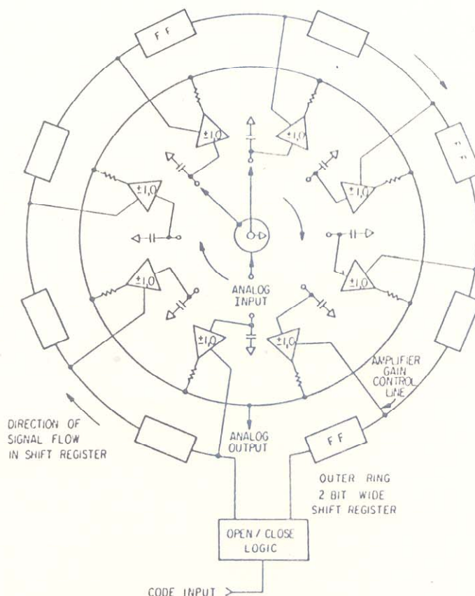
Figure 4. Block diagram of analog ring decoder.
