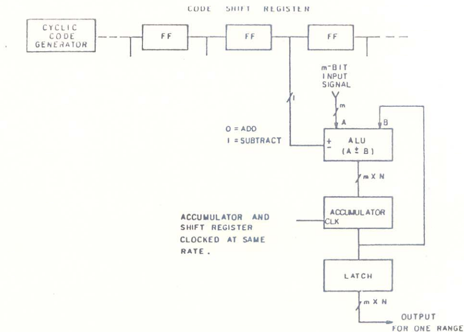
Figure 3. Decoder using correlator architecture uses one channel per range (one channel shown).
