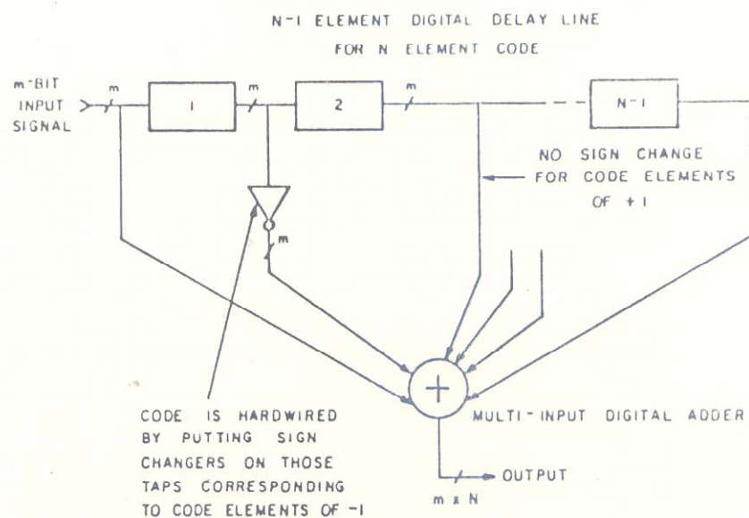
Figure 1. Transversal filter decoder for code length N .
