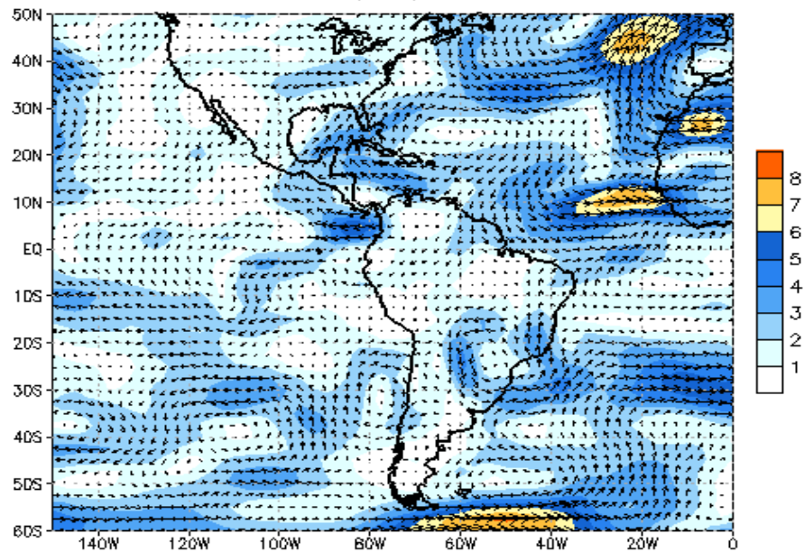
850 hPa Vector Wind Anomalies ( \text{ms}^{-1} ) 02 DEC 2018 - 31 DEC 2018
