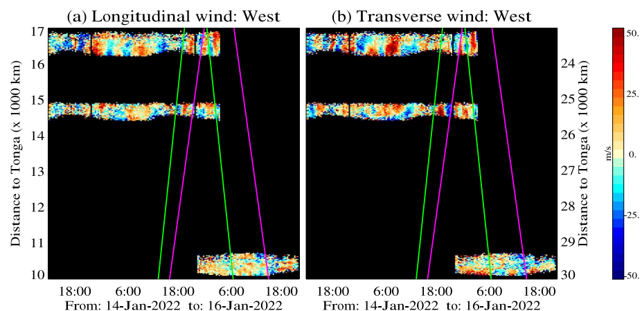
Figure 11. Similar to Figure 10 but for westward propagating perturbations.
