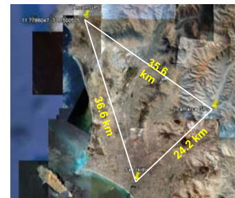
Fig 6. stations used in March 2009 Gravity Wave Campaign
