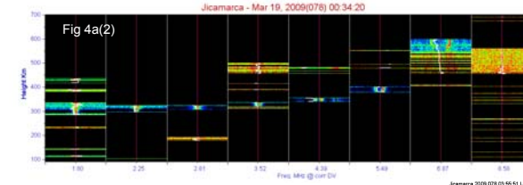
The VIPIR is operated in a mode which transmits 8 frequencies with 128 repeats; this makes each frequency observed at sampling interval of 0.064 seconds. These series is used to calculate the doppler spectra and mean velocities as shown in figures 4a(2), d(2) and 5b. The scale of the spectrum is from -4 to 4 Hz for each frequency and the mean velocity scale varies from -50 m/s to 50 m/s.
